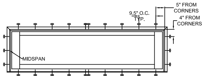
TYPICAL ELEVATION WITH FASTENER SPACING
