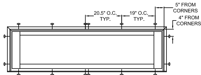
TYPICAL ELEVATION WITH FASTENER SPACING
